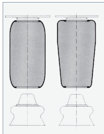
Cylindrical Air spring
